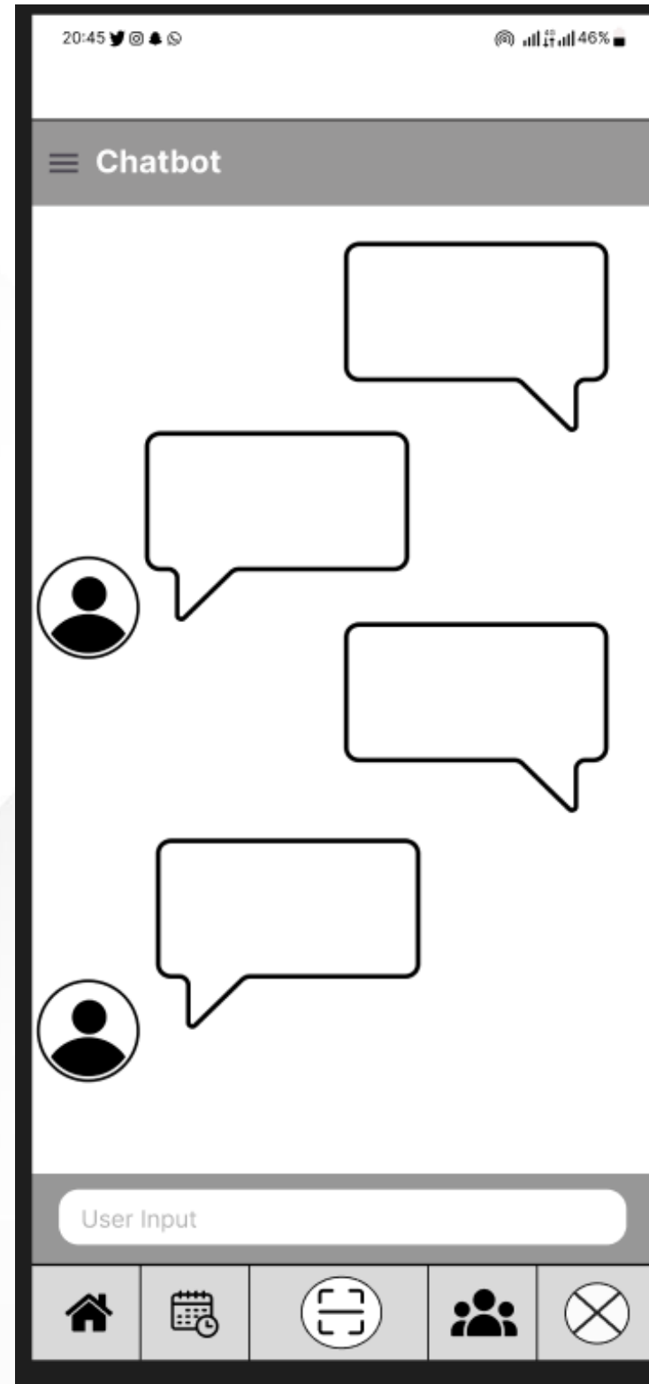
Expanded chatbot
