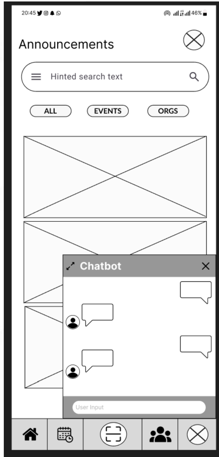
Chatbot
