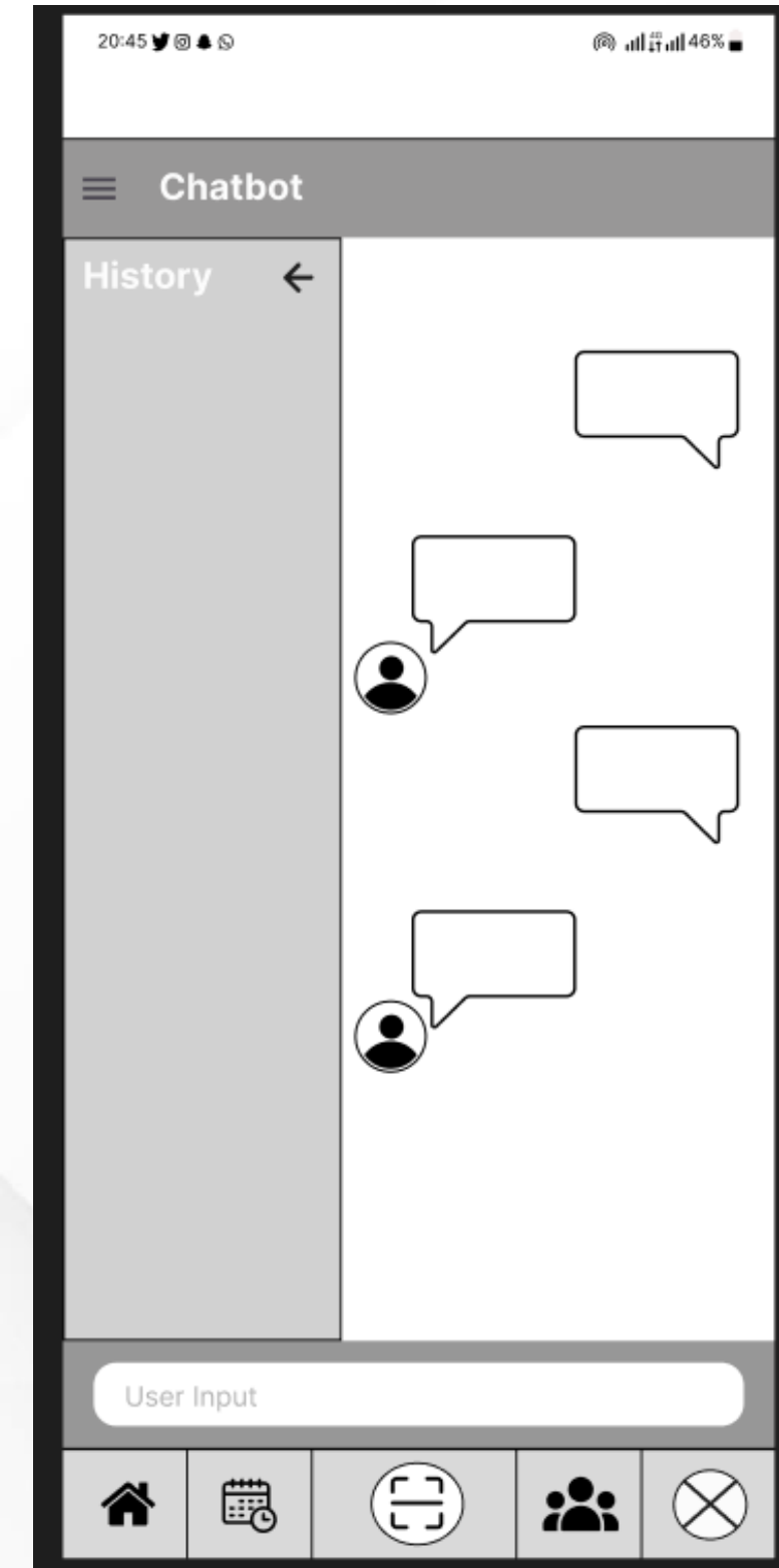
History chatbot
